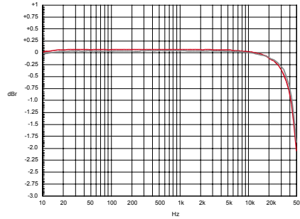
Figure 7.1 Gain vs. frequency ( Q-POWER 4/Q-POWER 6, Q-POWER 10 ) (Measurements of a typical performance)
