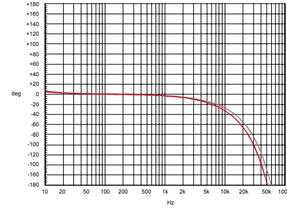
Figure 7.3 Phase vs. frequency ( Q-POWER 4/Q-POWER 6, Q-POWER 10 ) (Measurements of a typical performance)
