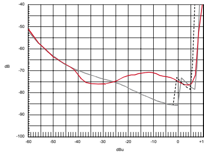
Figure 7.2 THD @ 1 kHz, 8 Ω vs. input voltage ( Q-POWER 4 / Q-POWER 6, Q-POWER 10 ) (Measurements of a typical performance)
