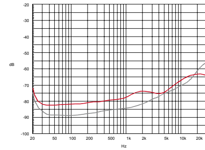
Figure 7.4 THD vs. frequency, 10 dB below clip, 8 Ω ( Q-POWER 4/Q-POWER 6, Q-POWER 10 ) (Measurements of a typical performance)
